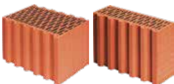
Porotherm 38 P+W Porotherm 38 1 / 2 P+W
